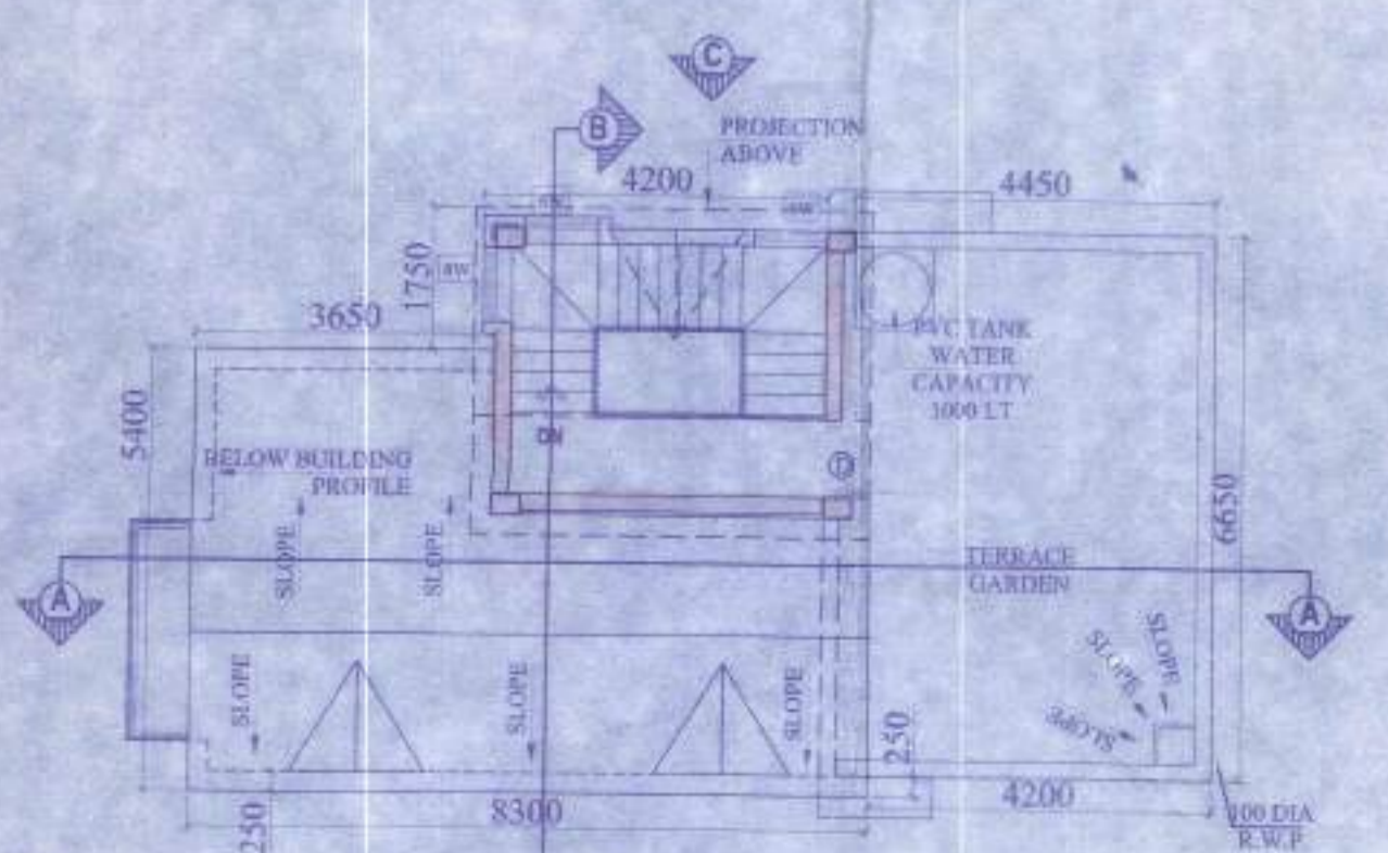
ROOF PLAN
